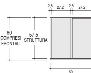
Terminale con anta e ripiani / Terminal with door and shelves
